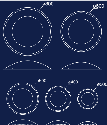
PF 314 GG = 2X R7s 100W OU E27 Ø600MM - NICO = Ø570MM
