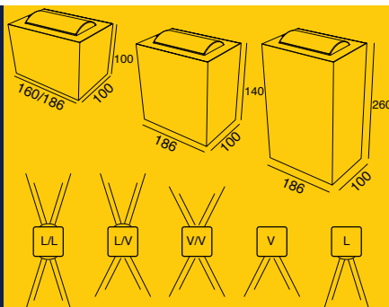
AR 105 - 1X R7s 78MM - PROF. 160MM
